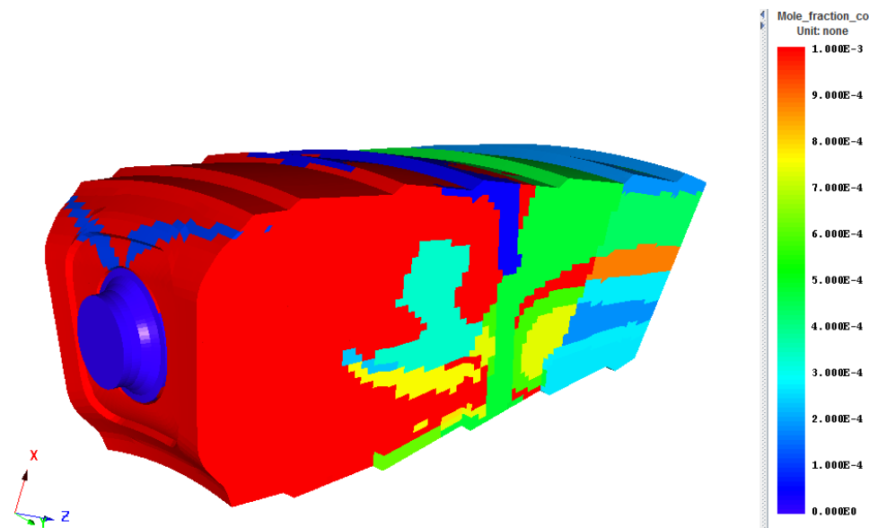
Figure 2. CO emissions on the combustor geometry.
