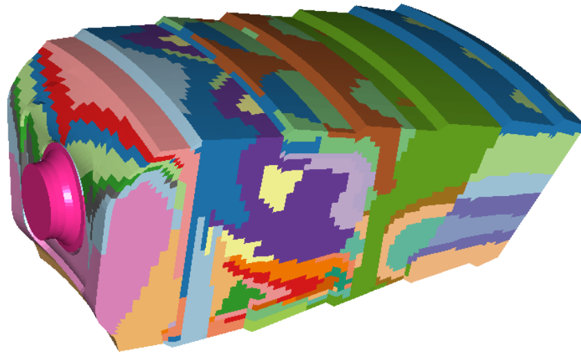
Figure 1. Reactor Zones in ENERGICO.
